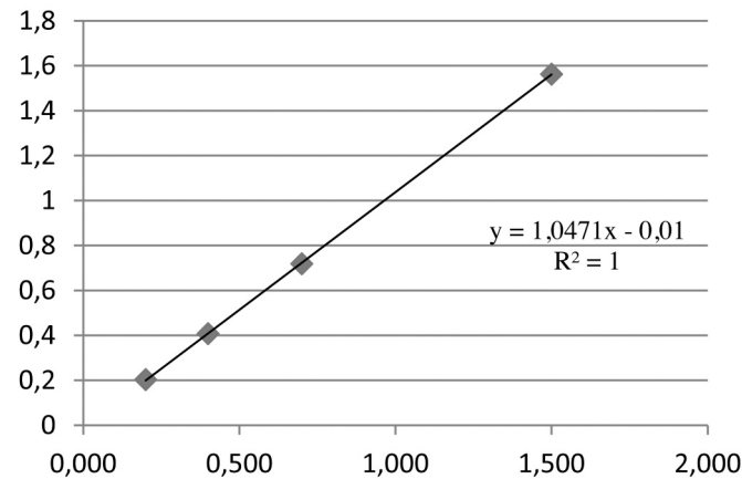
Figure 2 The calibration curve using LNE standard solutions and LNE simulator system
