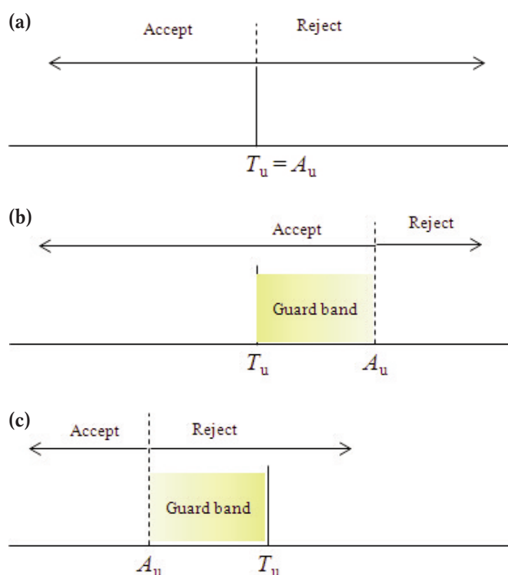
Figure 1: Acceptance or rejection of an item on the basis of a measurement result. T_u is an upper tolerance limit with which a measured property must comply (the true value must be less than T_u ). A_u is the upper acceptance limit of the measured value. (a) shared risk (or simple acceptance) where the tolerance and acceptance limits are equal; (b) guarded acceptance, which reduces the producer's risk; (c) guarded rejection, which reduces the consumer's risk. The nomenclature follows from guidance document JCGM 106:2012.
