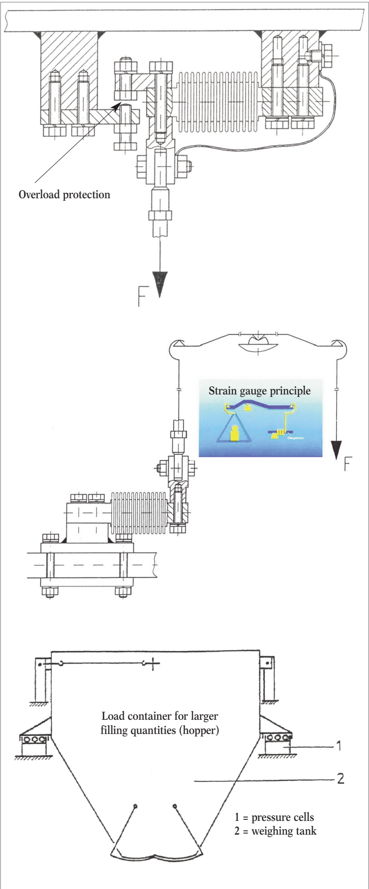
Figure 3: Examples of LC internal fittings
