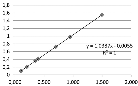
Figure 4 The calibration curve using INM standard solutions and INM simulator system
