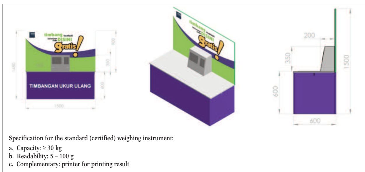
Figure 1: Dimensions and specifications of the weighing scales re-checker unit
