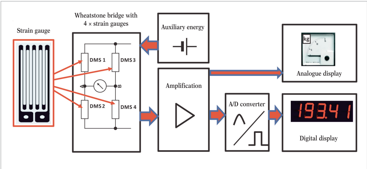
Figure 4: Analogue/digital conversion
